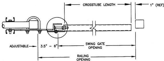
TOP VIEW OF SWING GATE WITH INLINE MOUNTING
