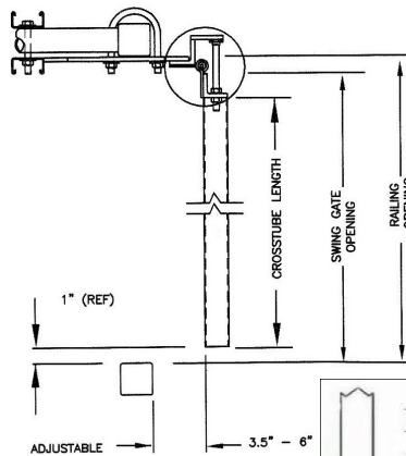
TOP VIEW OF SWING GATE WITH 90° MOUNTING
